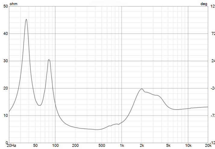
HORN IMPEDANCE
