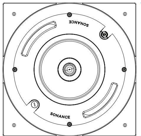
Loudspeaker Square Adapter Front 13.27" x 13.27" (337mm x 337mm)
