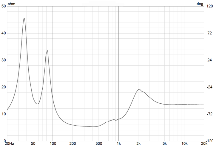
COLLAR IMPEDANCE
