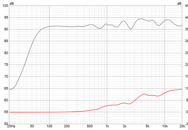
HORN SPL
