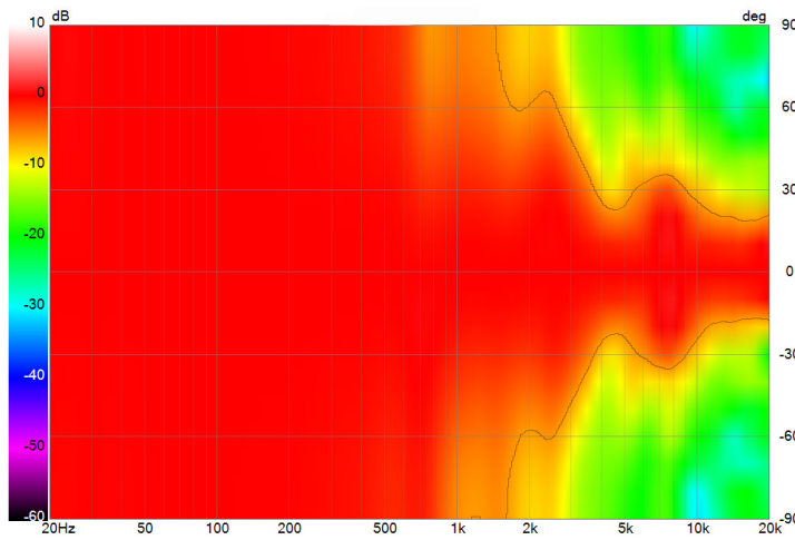
HORN DIRECTIVITY
