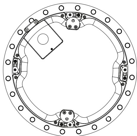
Loudspeaker Back 11.5" (292mm)
