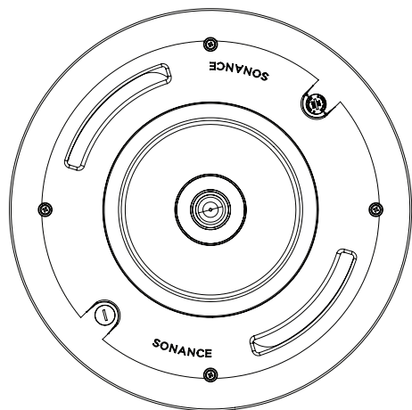
Loudspeaker Front 13.27" (337mm)
